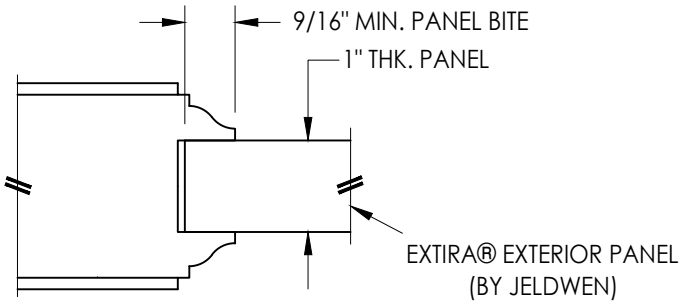
P1 WOOD PANEL DETAIL
