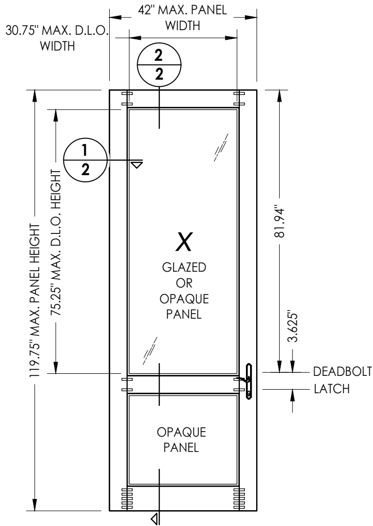
40 3/4 GLAZED OR OPAQUE DOOR PANEL UPSTATE DOOR
