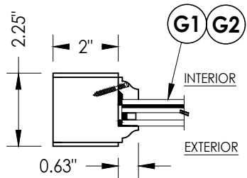
1 3 HORIZONTAL CROSS SECTION
