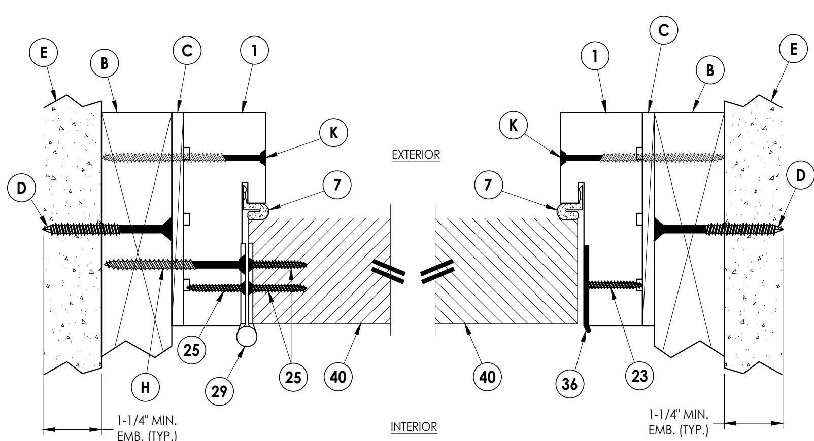
1 5 HORIZONTAL CROSS SECTION 2X Buck Construction
