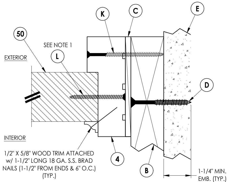
3 5 HORIZONTAL CROSS SECTION 2X Buck Construction
