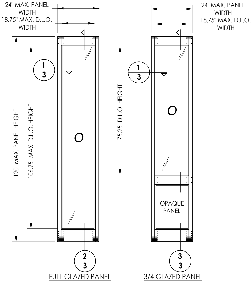
50 SIDELITE PANELS UPSTATE DOOR
