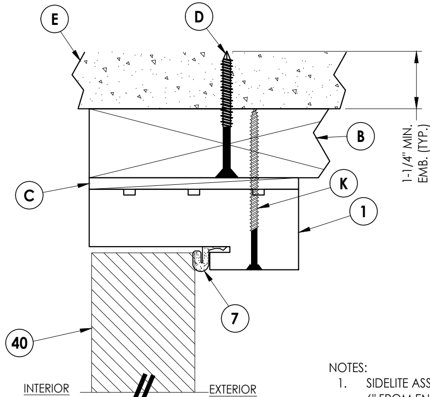
4 5 VERTICAL CROSS SECTION 2X Buck Construction
