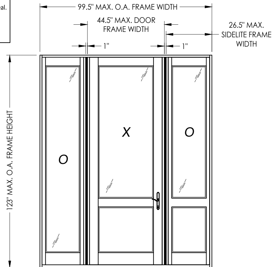
CONTINUOUS HEAD & SILL
