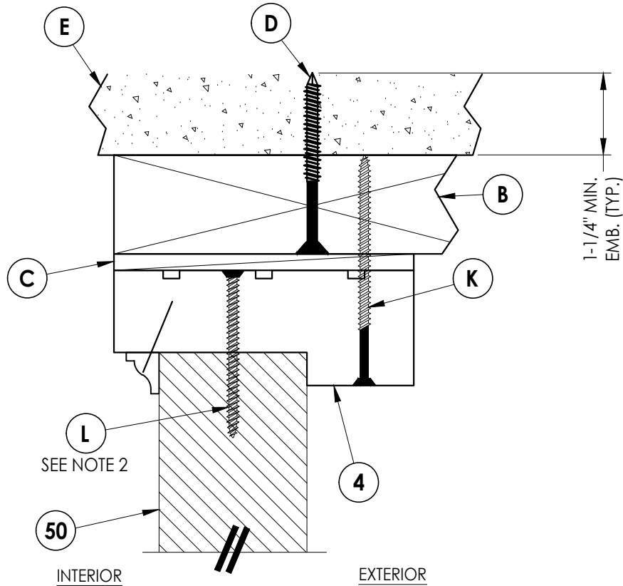
5 5 VERTICAL CROSS SECTION 2X Buck Construction
